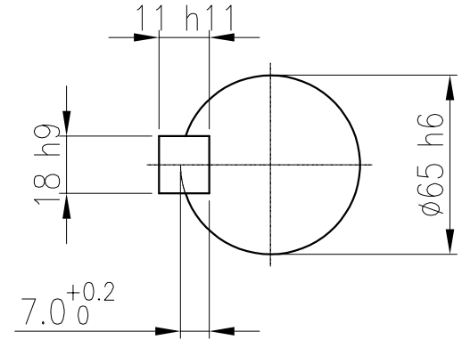
OUTPUT SHAFT KEY 18 x 11 x 54
